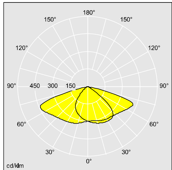
22676676_JET_3_LED_LED_730_75W_SPD15_CL2_L60_GREY.lgt
