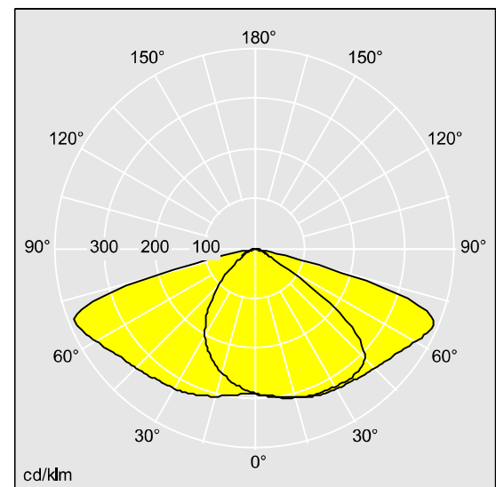
22676680_JET_3_LED_LED_730_215W_SPD15_CL2_L60_GREY.lgt
