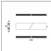
Code 0.26865.0031 - Electromechnical connection - Pendant- 1000mm - Power
