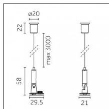
Code 0.26877.0P00 - Suspension accessory with stabilizer - short brackets (2x)
