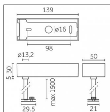
Code 0.26831.0P12 - Suspension set with 1,5m tige - short brackets (2x)
