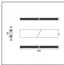
Code 0.26864.0031 - Electromechnical connection - Pendant- 500mm - Power
