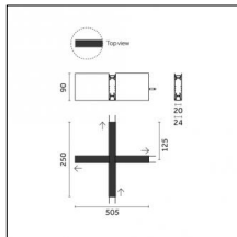
Code 0.26868.0012 - Electromechanical connection - Pendant-X - 250x250mm - Continuous
