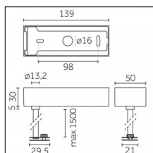
Code 0.26831.0P31 - Suspension set with 1,5m tige - short brackets (2x)
