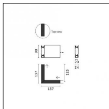
Code 0.26866.0031 - Electromechnical connection - Pendant- L - 125x125mm - Continuous
