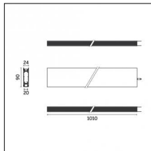
Code 0.26865.0012 - Electromechnical connection - Pendant- 1000mm - Power
