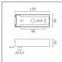
Code 0.26881.0012 - Surface trim base (without cable)
