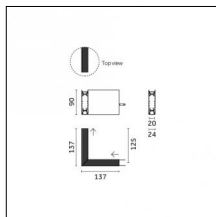
Code 0.26866.0012 - Electromechnical connection - Pendant- L - 125x125mm - Continuous
