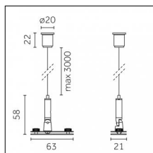
Code 0.26878.0P00 - Suspension accessory with stabilizer - long bracket
