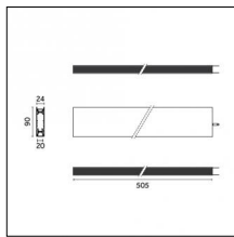
Code 0.26864.0012 - Electromechnical connection - Pendant- 500mm - Power
