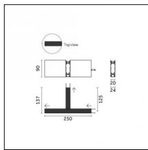
Code 0.26867.0031 - Electromechanical connection - Pendant-T - 250x125mm - Continuous
