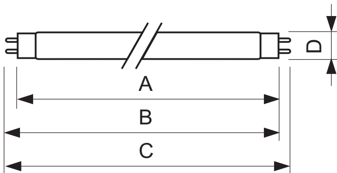
TL-D Colored 18W Red 1SL
