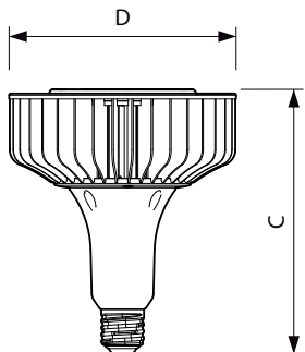
TrueForce LED HIL ND 150-400W E40 840 60D
