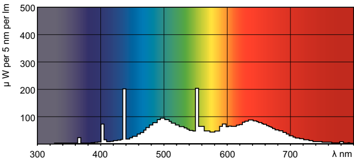
LDPO_TL-D9HCR_950-Spectral power distribution Colour
