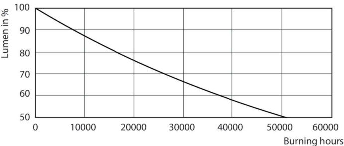
Lumen Maintenance Diagram - MAS LED spot VLE D 3.7-35W GU10 940 60D
