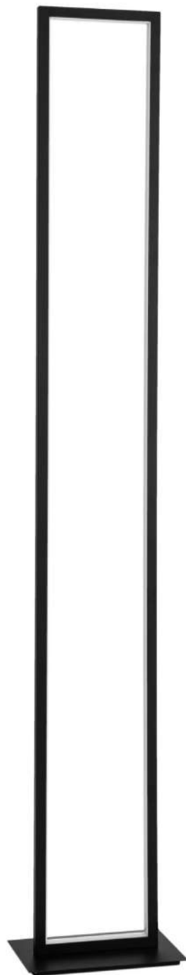
WENNA - 9500812 20.5 16 26 24 153 Matt Black Aluminium & Acrylic LED 36 Watt 230 Volt 2150Lm 3000K IP20 L: 26 W: 16 H: 153 cm LED WARM WHITE A++ A DRIVER INCL.
