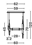
ZIMBA - 9862873 Dimmable Gold Brass Metal White Glossy Glass LED 54 Watt 230 Volt Lm 3000K IP20 L: 60 W: 60 H 1 : 70 H 2 : 120 cm LED WARM WHITE A++-A DRIVER INCL.
