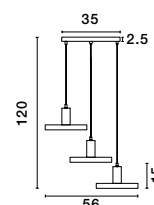
GARNI - 9417051 Black Metal Outside & Gold Inside Black Pvc Wire LED E27 3x12 Watt 230 Volt IP20 Bulb Excluded D: 56 H: 120 cm
