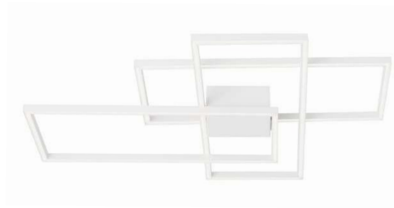
BILBAO • 9977001 Dimmable White Aluminium & Acrylic LED 55 Watt 230 Volt 3550Lm 3000K IP20 L: 90 W: 67 H: 8.5 cm
